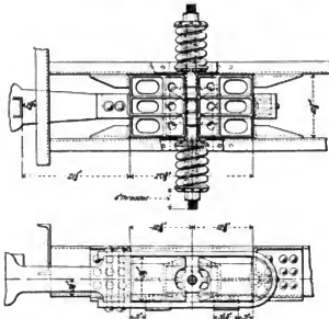
Figs. 3927-3928. Cardwell Friction Draft Gear, Type C-1.
